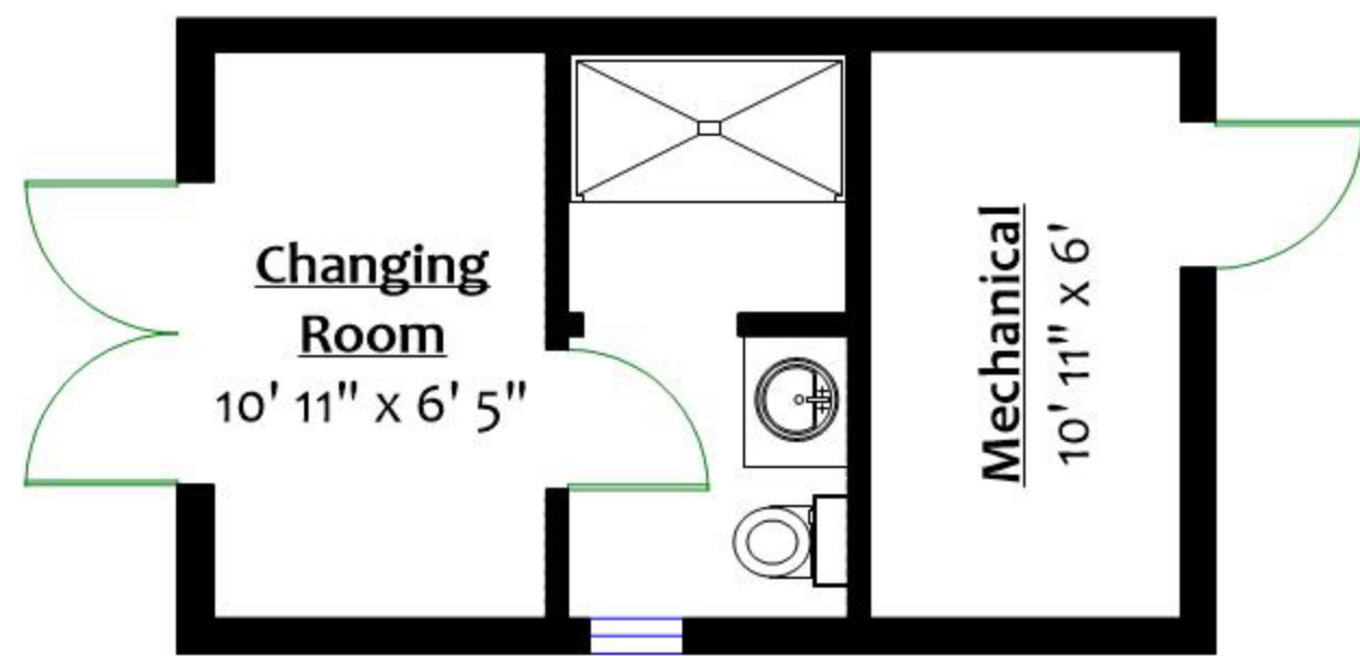
POOL HOUSE Floor Area: 242 Sq. Ft.
