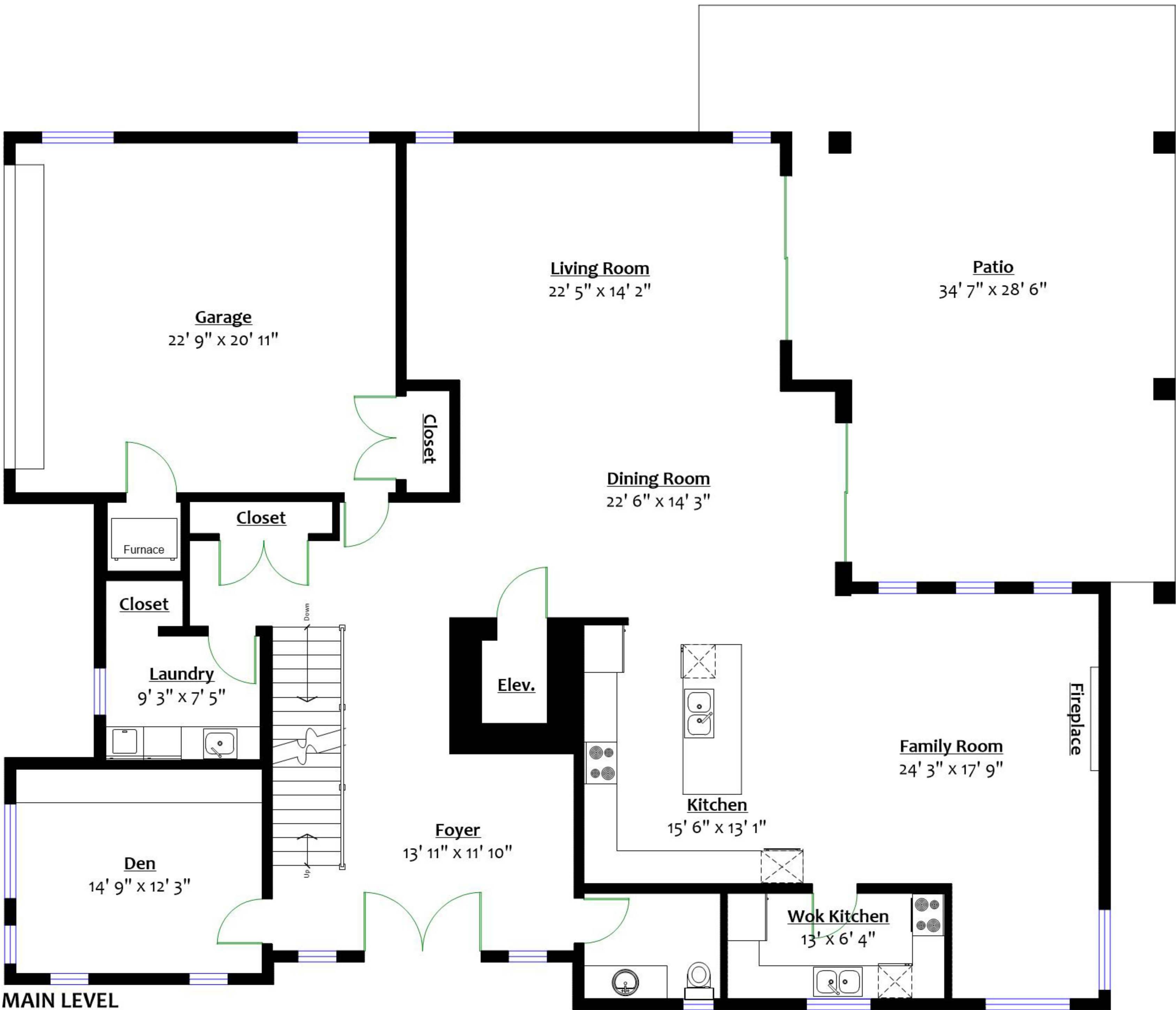
MAIN LEVEL Floor Area: 2,313 Sq. Ft.
