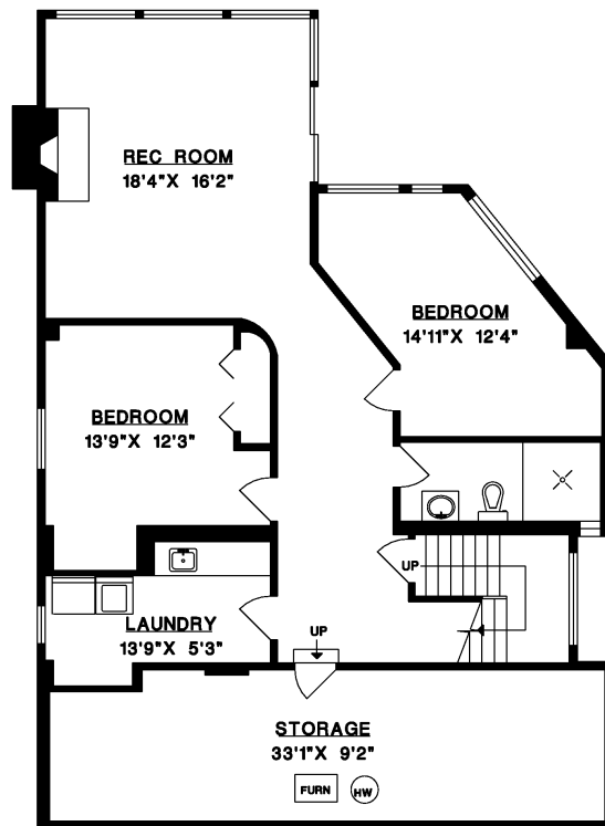
LOWER FLOOR
